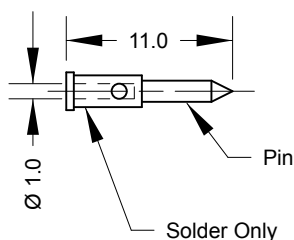
Pin and insulator arrangement
